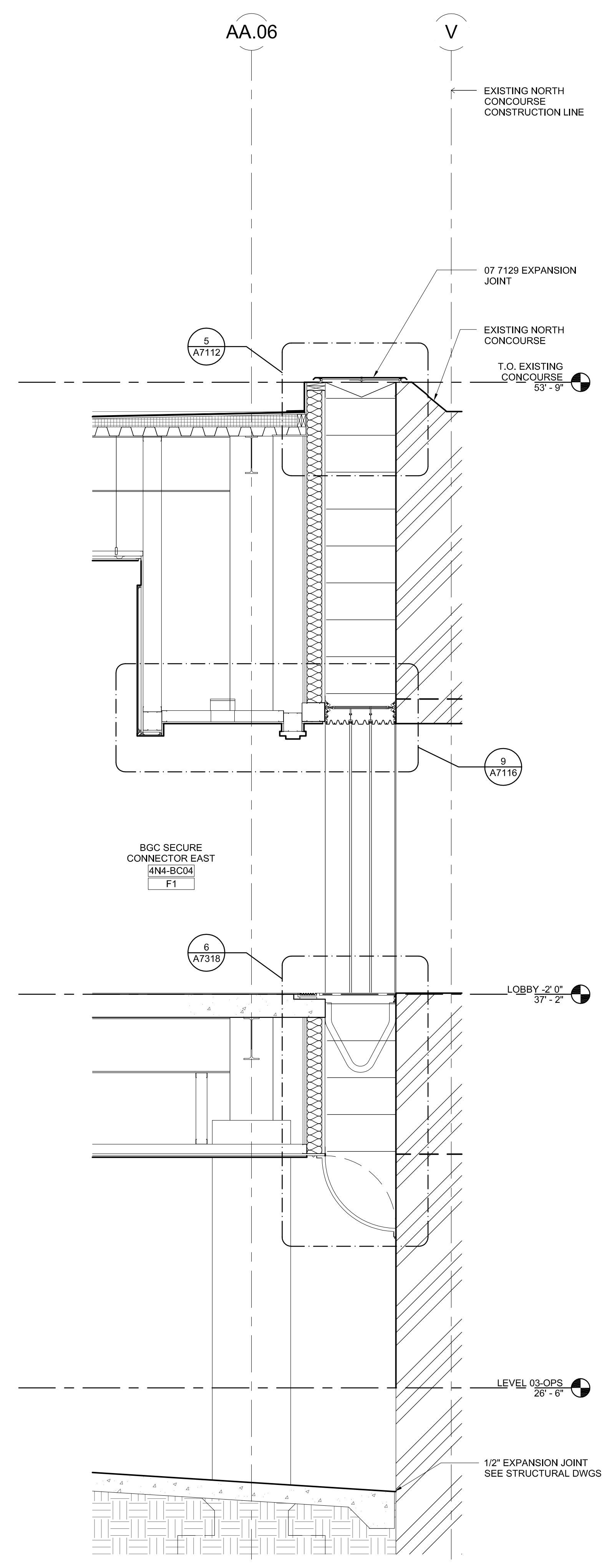
3 SECTION @ GATE 123 BUILDING A6118/A6217 1/2" = 1'-0"
