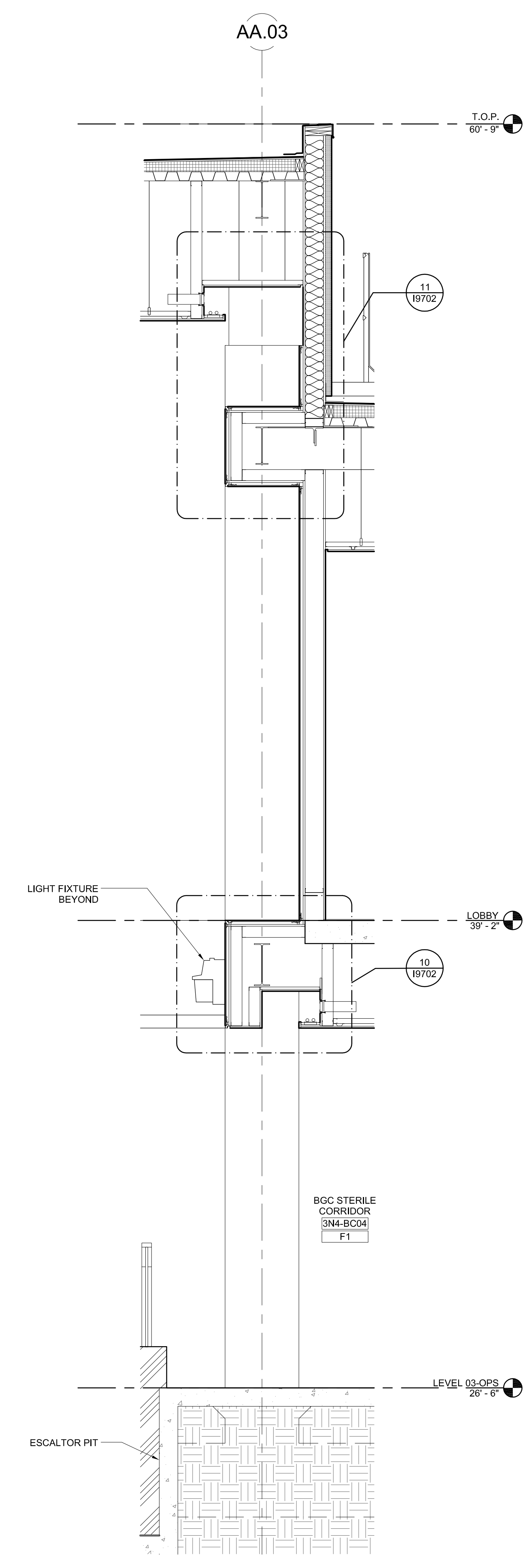
4 SECTION @ BGC STERILE CORRIDOR A2843/A6217 1/2" = 1'-0"
